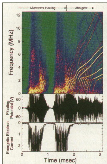
Storm in a bottle. Microwave heating excites high-frequency waves in a laboratory plasma (top), which periodically unleashes bursts of electrons (bottom). A similar process may take place during storms in Earth's magnetosphere.
