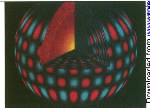
Internal noise. Sound waves traveling through a star like the sun, shown in this computer model, compress (red) and elevate (blue) surface areas in a pattern that reveals interior details.
